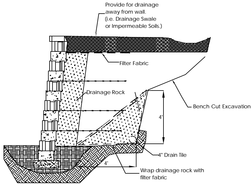
Typical Heel Drain Option
