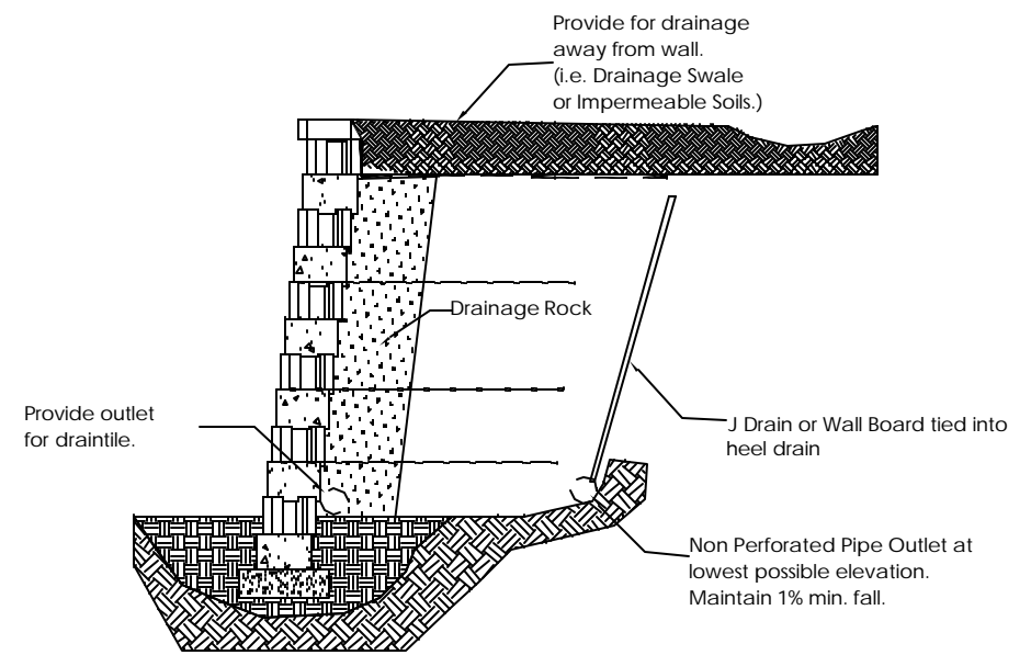
Typical J Drain/Wall board option
