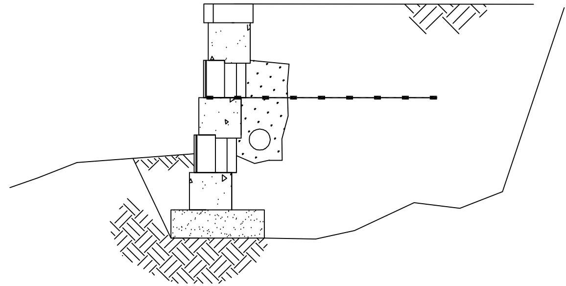
Straight Classic Alliance Typical cross section
