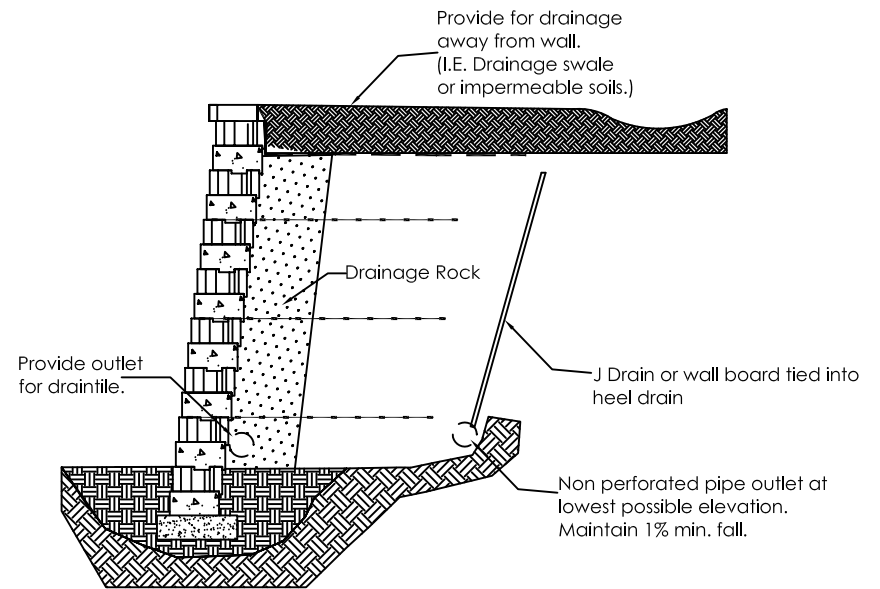
Typical J Drain/Wall Board Option
